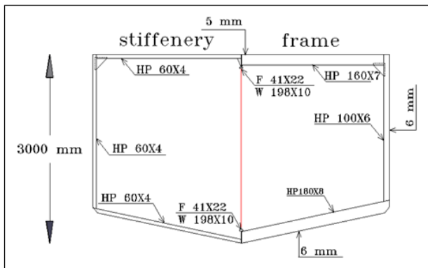
Fig. 5. Final dimension drawn boat
