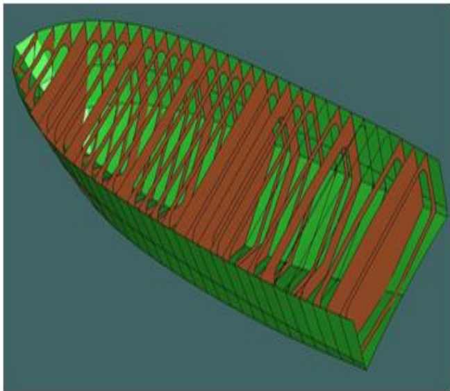
Fig. 4. Workshop drawing of the structure
