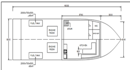
Fig. 3. Plan view of the second floor
