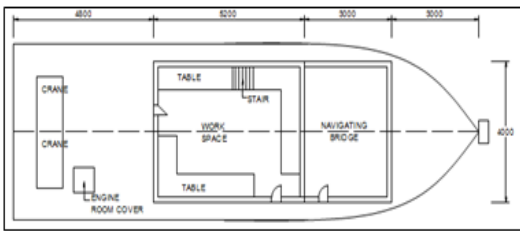
Fig. 2. Plan view of first floor
