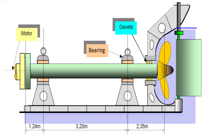
Fig. 6 – Shaft and Propeller Diagram
