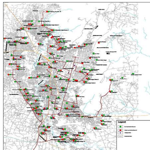
Fig.2: Existing Water Supply System Proposals under Bisalpur Project
