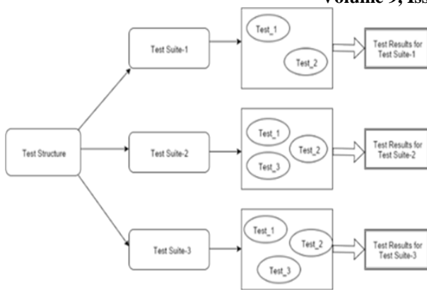
Fig.3. Test Suites
