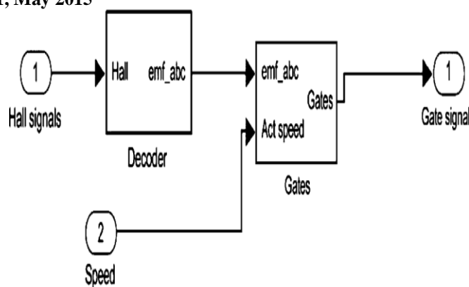
Fig 5 Modeling of Controller.
