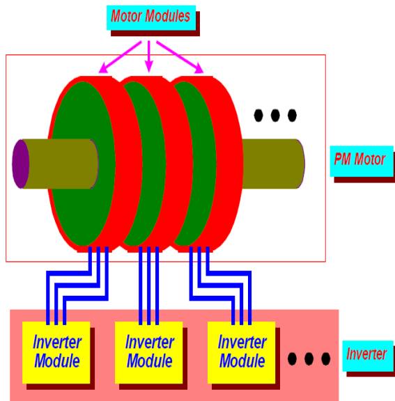
Fig 1 Modular inverter and modular motor drive system configuration.
