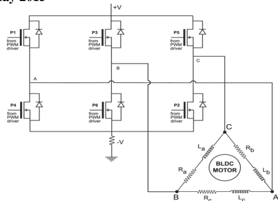
Fig 2 Equivalent Circuit of power stage of BLDC motor.
