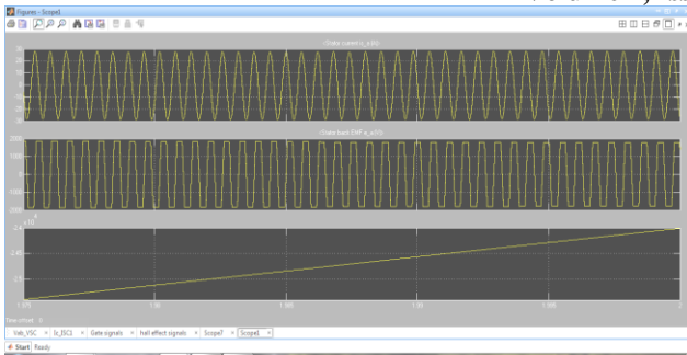
Fig 10 Stator Current, Stator Back EMF, Rotor Speed(rpm)
