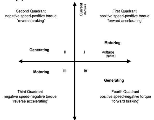
Fig 3 Four Quadrants of operation.
