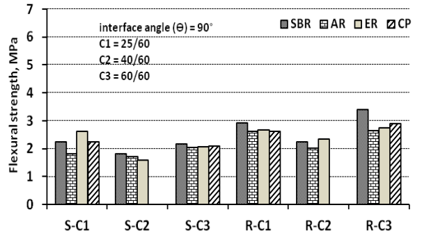
Fig. 10 Flexural strength results of different binder materials (as-cast, rough specimens, \theta=90^\circ ).
