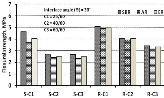
Fig. 7 Flexural strength results of different binder materials (as-cast, rough specimens, \theta=30^\circ ).
