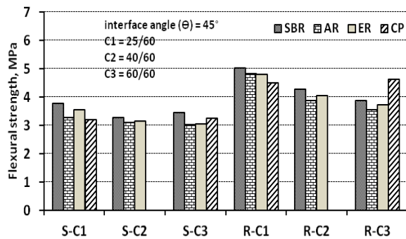
Fig. 8 Flexural strength results of different binder materials (as-cast, rough specimens, \theta=45^\circ ).
