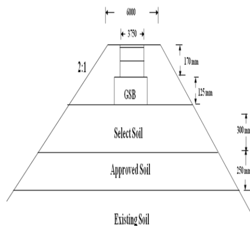
Fig.1 Normal section of rural road
