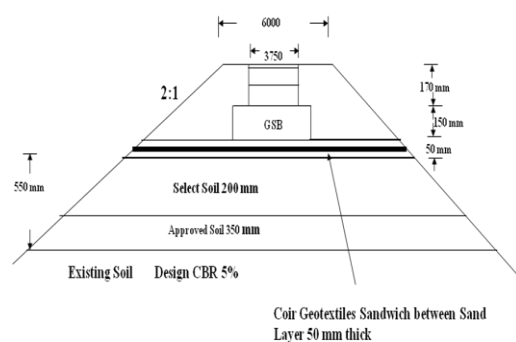
Coir Geotextiles directly placed over the select Soil (200) (Case-III)
