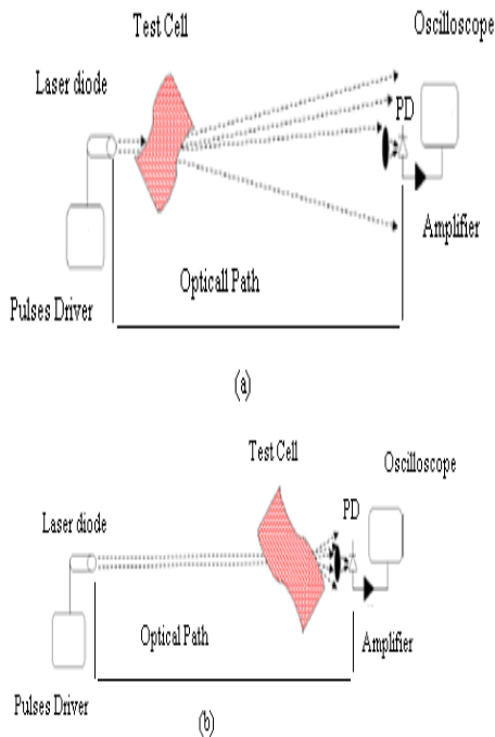
Fig 3. Sketch of diverted beams due to turbulence source positioned (a) near the transmitter and (b) near the receiver
