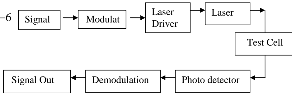
Fig 1. Block diagram of experiment setup
