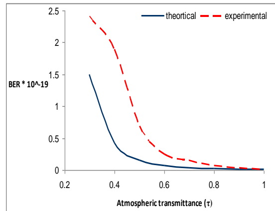
Fig 5 The theoretical and experimental of the BER as a function of atmospheric transmittance
