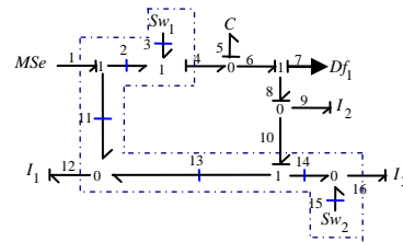
Fig 3. The acausal BG
