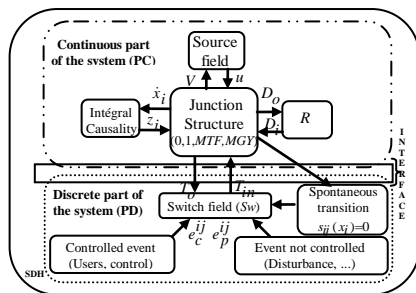
Fig 1. Structure junction
