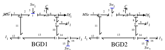
Fig 5. a) BGD1+dualization of sources (mode 1), b) BGD2+dualization of sources (mode 2)
