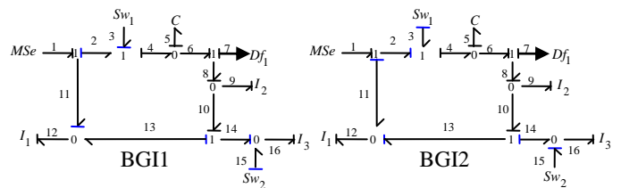
Fig 4. The BGI1 and BGI2
