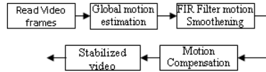
Fig.2.Proposed block diagram..
