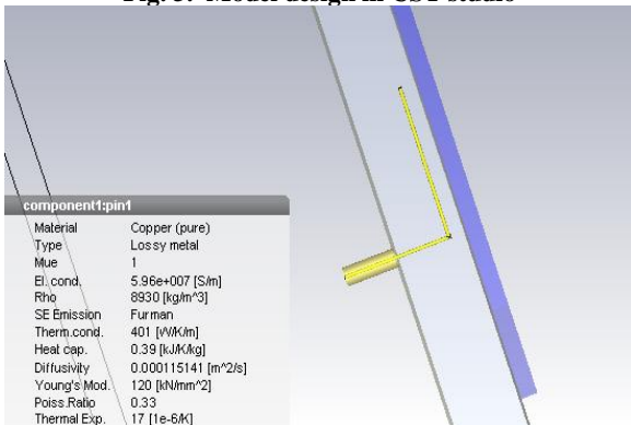
Fig. 4. Side view of model design in CST studio
