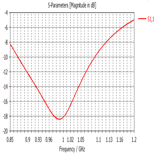
Fig. 9. Simulated |S11| parameter of proposed water dielectric patch antenna
