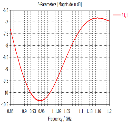
Fig. 5. Simulated |S_{11}| parameter of proposed water dielectric patch antenna
