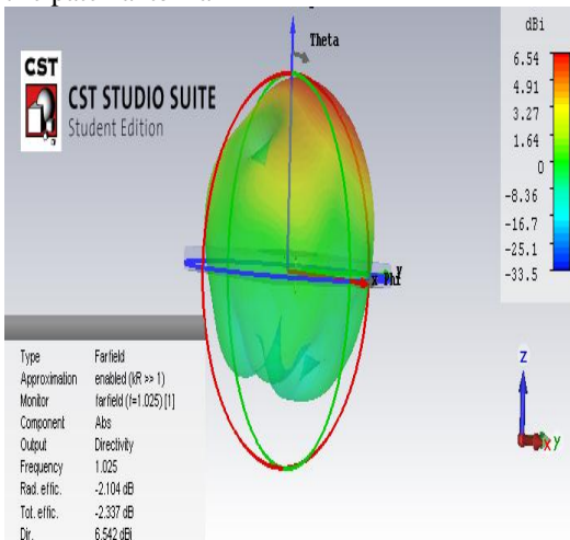
Fig. 11. Simulated 3D view far field directivity of water dense dielectric patch antenna
