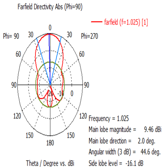
Fig. 6. Simulated radiation pattern of the proposed water dense dielectric patch antenna at the centre frequency of operating band.
