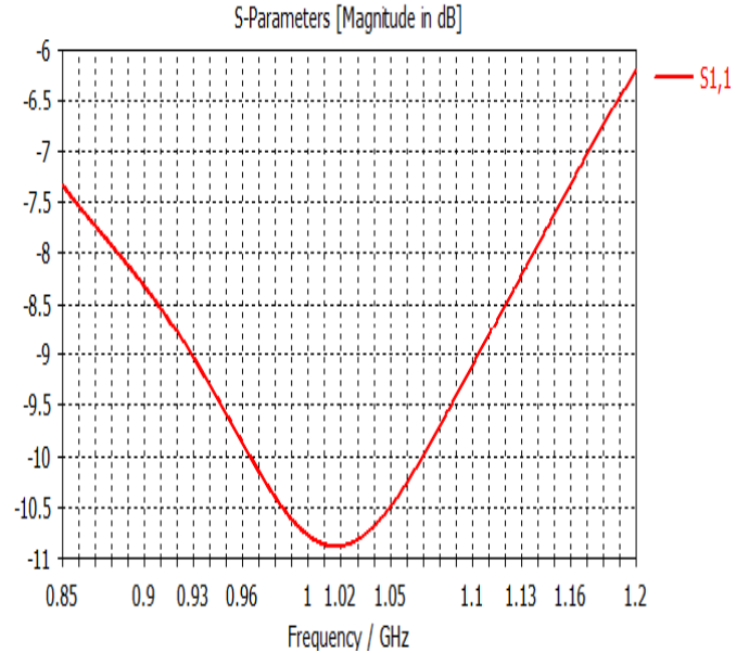
Fig. 7. Simulated |S_{11}| parameter of proposed water dielectric patch antenna
