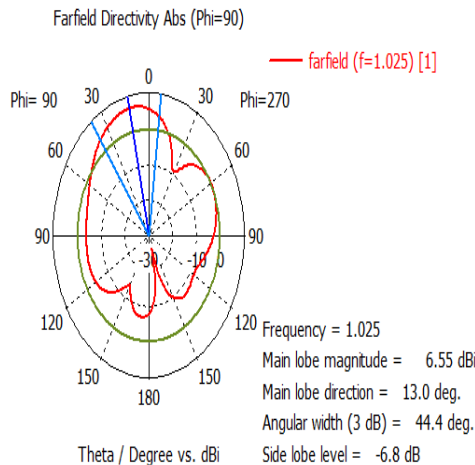
Fig. 10. Simulated radiation pattern of the proposed water dense dielectric patch antenna at the centre frequency of operating band.
