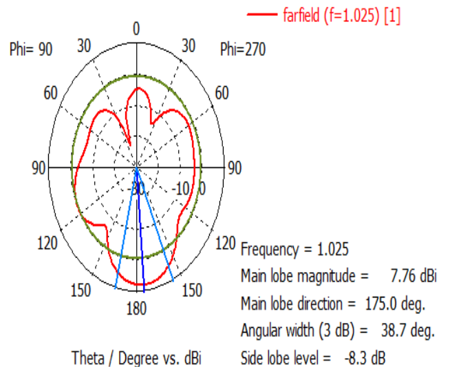
Fig. 8. Simulated radiation pattern of the proposed water dense dielectric patch antenna at centre frequency of the operating band.
