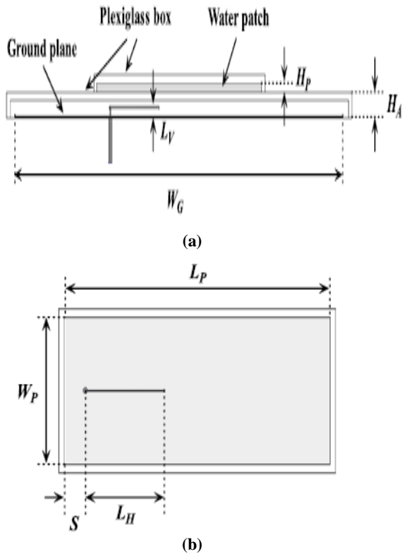
Fig. 2. Geometry of the L-probe fed water dielectric patch antenna (a) Side view (b) Top view [14]
