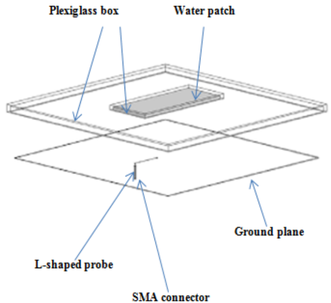
Fig. 1. Geometry of the L-probe fed water dielectric patch antenna [14]
