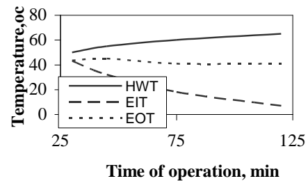
Fig.2 Temperature variation in the refrigeration cycle
