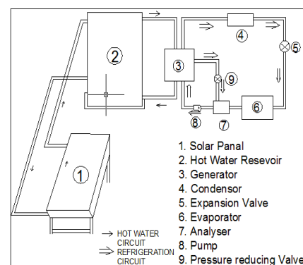
Fig.1 (b) Experimental set-up of Solar Cooling System
